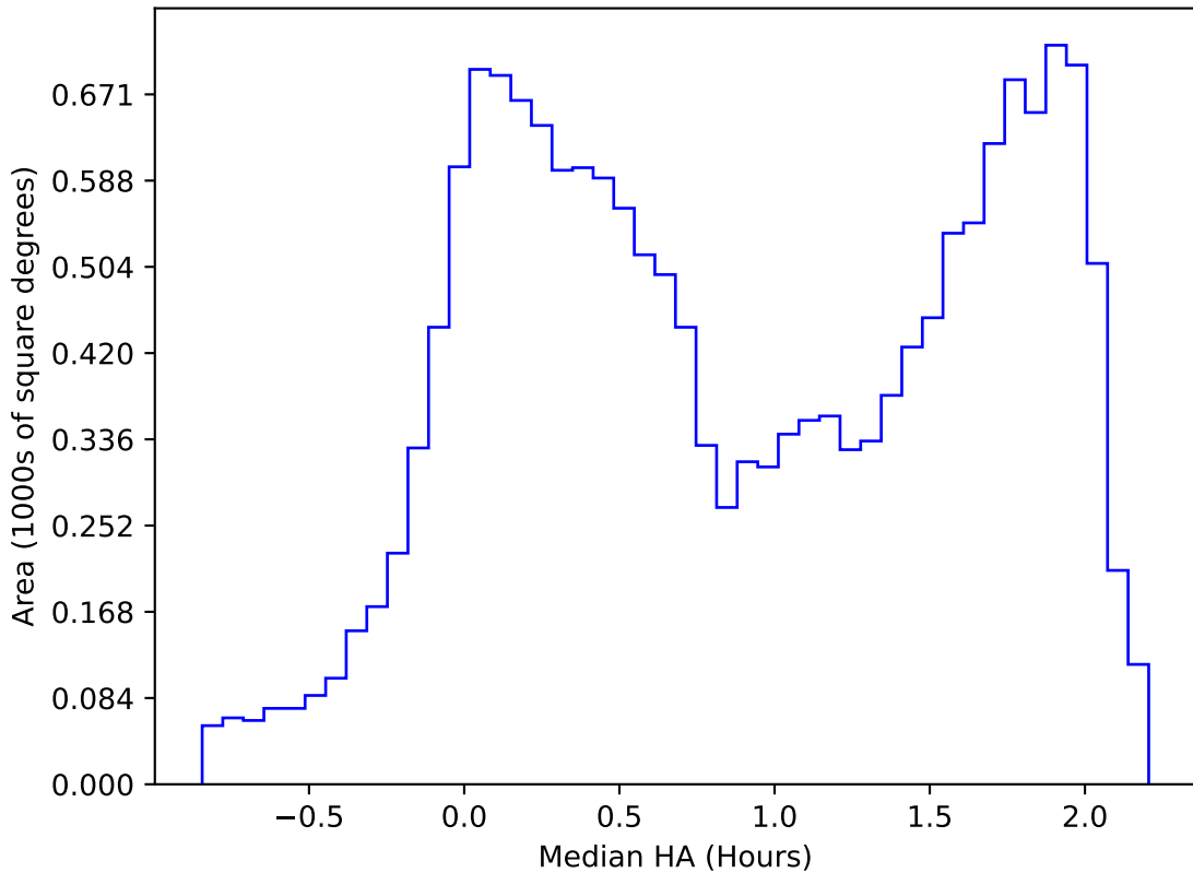
early_u_fpextra2.0_v3.4_10yrs WFD r band: Median HA
