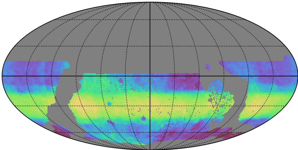
early_u_fpextra2.0_v3.4_10yrs WFD i band: Median HA
