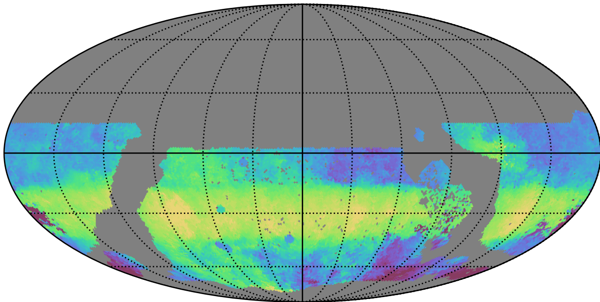
early_u_fpextra2.0_v3.4_10yrs WFD g band: Median HA
