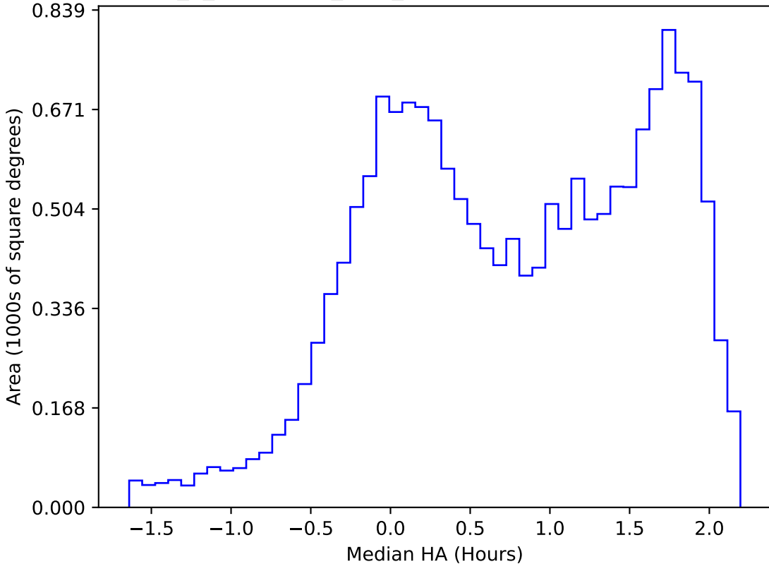
early_u_fpextra2.0_v3.4_10yrs WFD g band: Median HA
