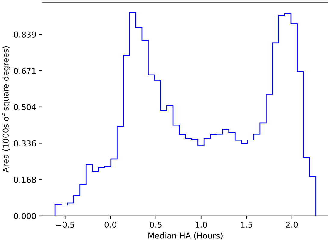
early_u_fpextra2.0_v3.4_10yrs WFD all bands: Median HA
