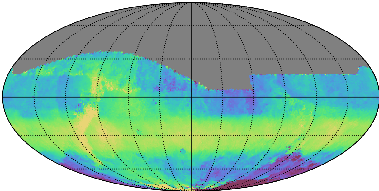
early_u_fpextra2.0_v3.4_10yrs All sky z band: Median HA
