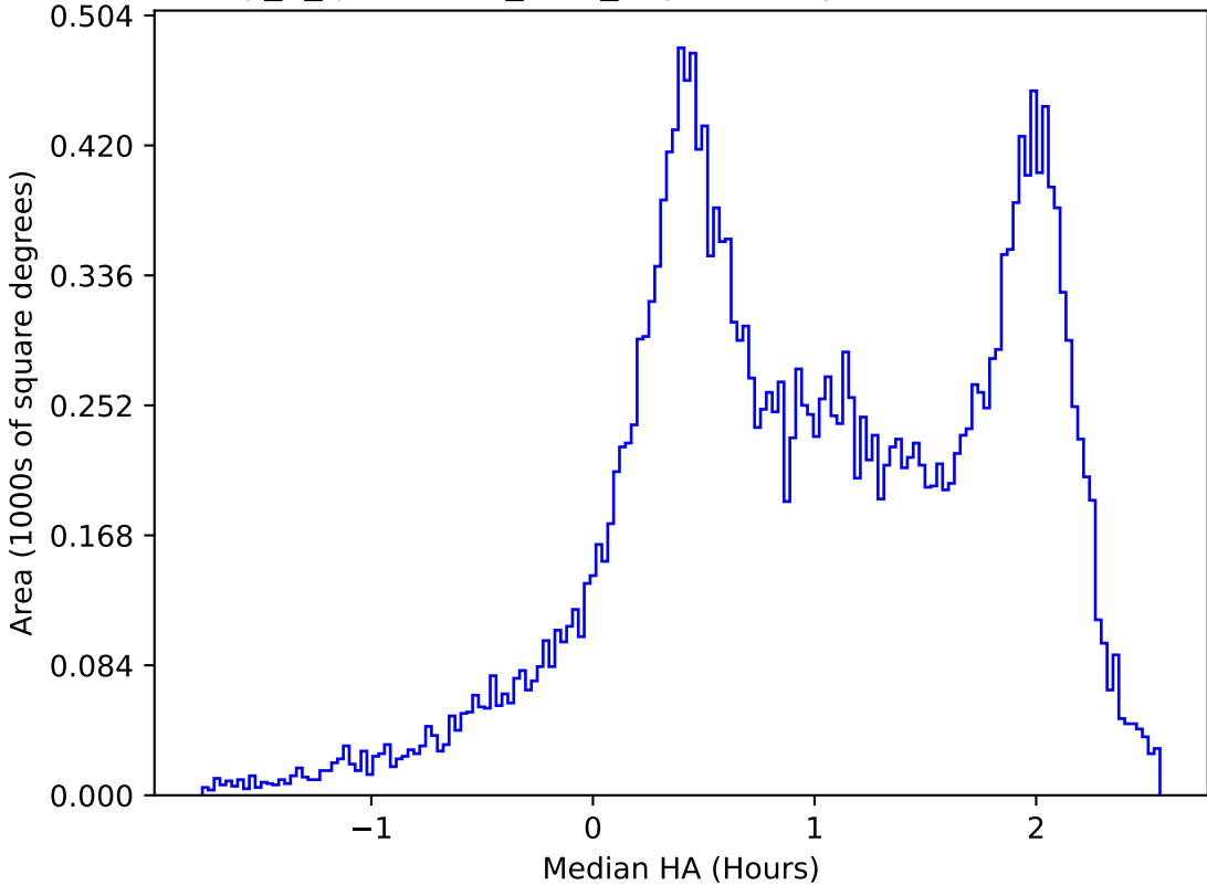
early_u_fpextra2.0_v3.4_10yrs All sky z band: Median HA
