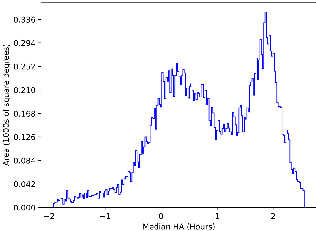
early_u_fpextra2.0_v3.4_10yrs All sky u band: Median HA
