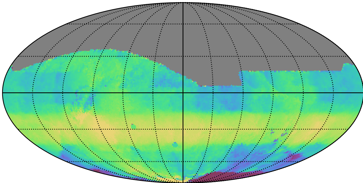
early_u_fpextra2.0_v3.4_10yrs All sky r band: Median HA
