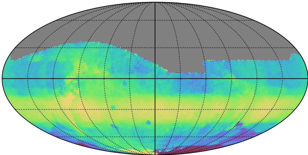
early_u_fpextra2.0_v3.4_10yrs All sky i band: Median HA
