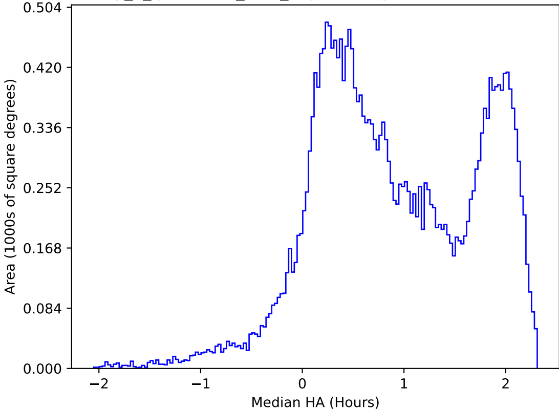
early_u_fpextra2.0_v3.4_10yrs All sky i band: Median HA
