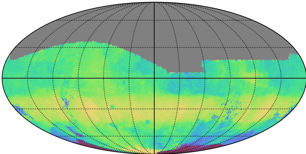
early_u_fpextra2.0_v3.4_10yrs All sky g band: Median HA
