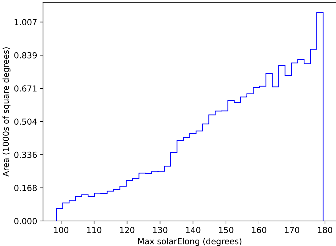
early_u_fpextra2.0_v3.4_10yrs WFD z band: Max solarElong
