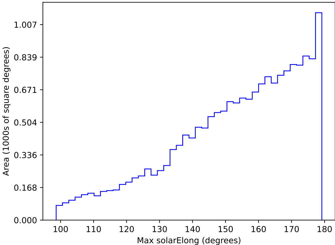
early_u_fpextra2.0_v3.4_10yrs WFD y band: Max solarElong
