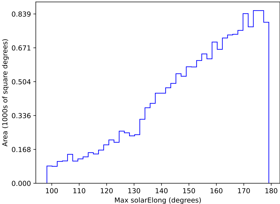
early_u_fpextra2.0_v3.4_10yrs WFD u band: Max solarElong
