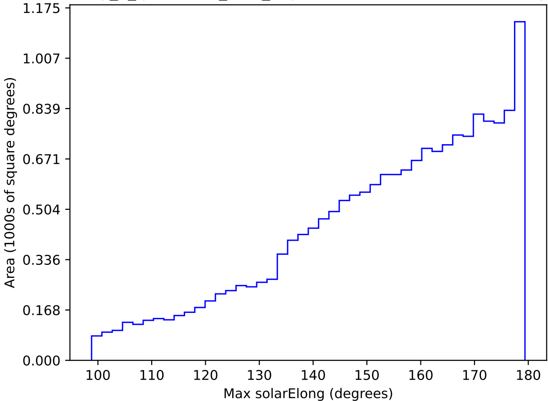
early_u_fpextra2.0_v3.4_10yrs WFD r band: Max solarElong
