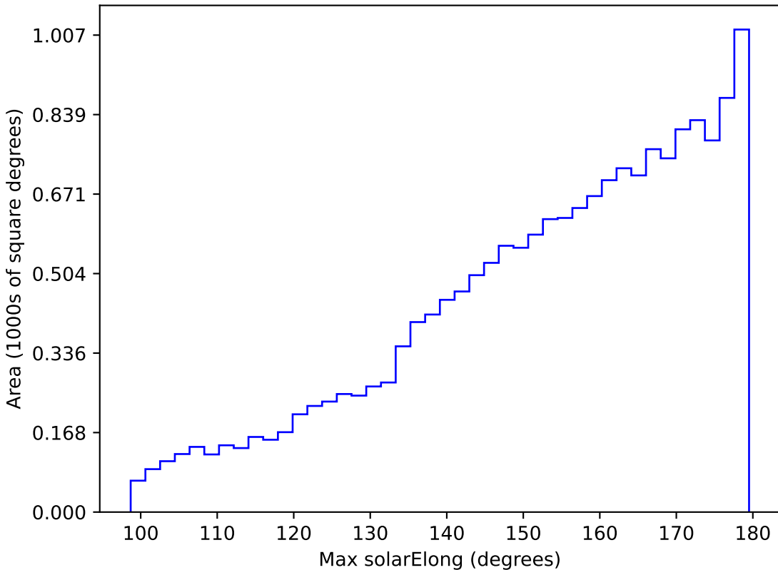
early_u_fpextra2.0_v3.4_10yrs WFD i band: Max solarElong
