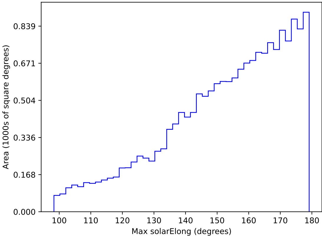
early_u_fpextra2.0_v3.4_10yrs WFD g band: Max solarElong
