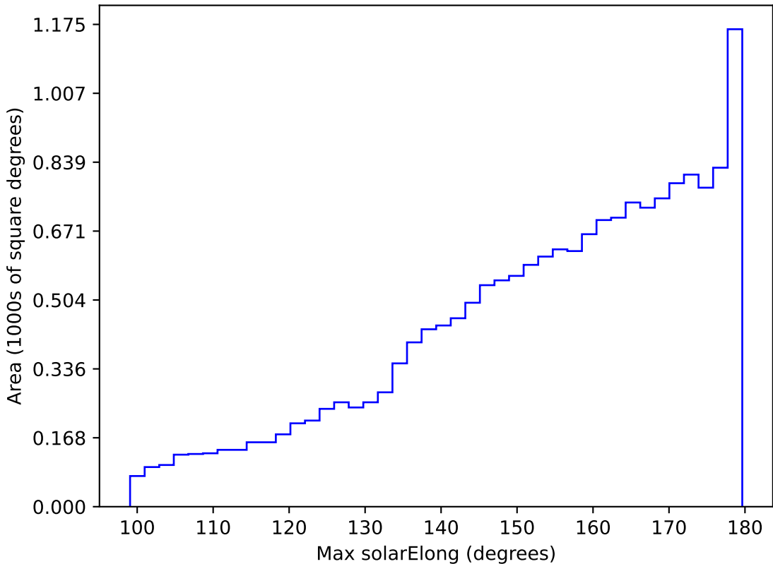
early_u_fpextra2.0_v3.4_10yrs WFD all bands: Max solarElong
