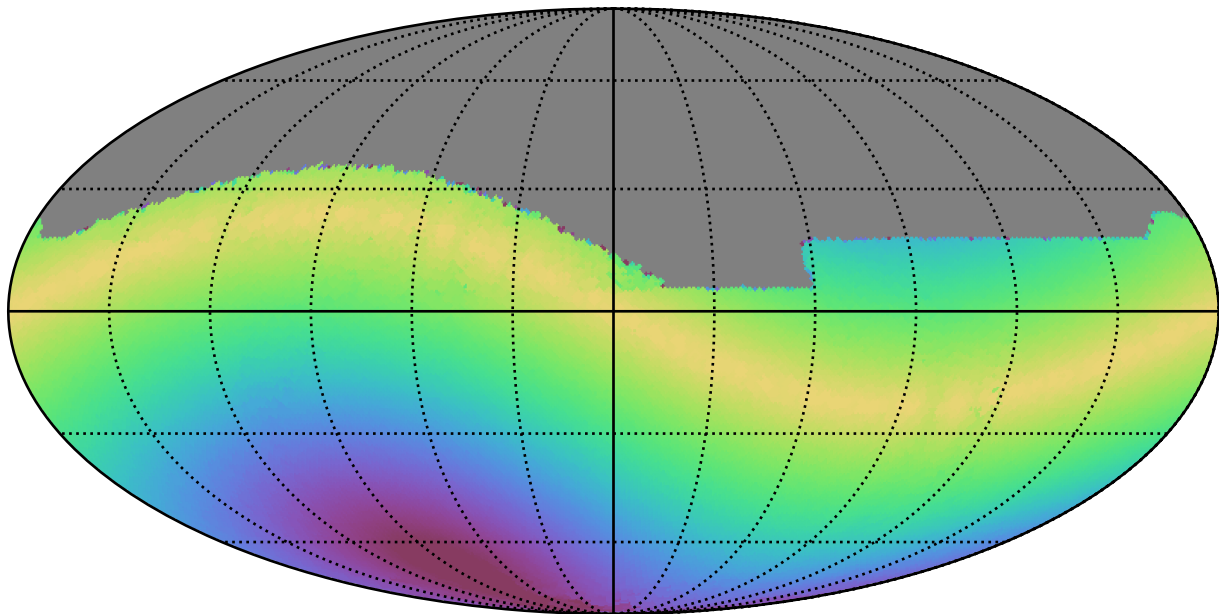
early_u_fpextra2.0_v3.4_10yrs All sky z band: Max solarElong
