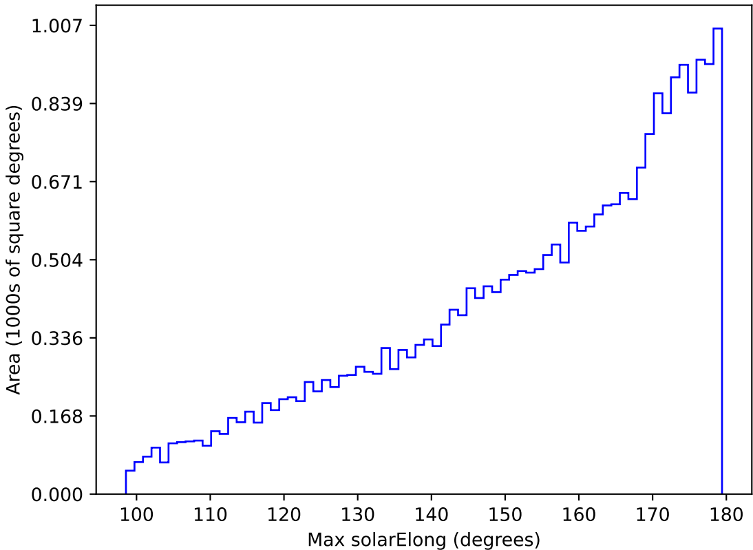
early_u_fpextra2.0_v3.4_10yrs All sky z band: Max solarElong
