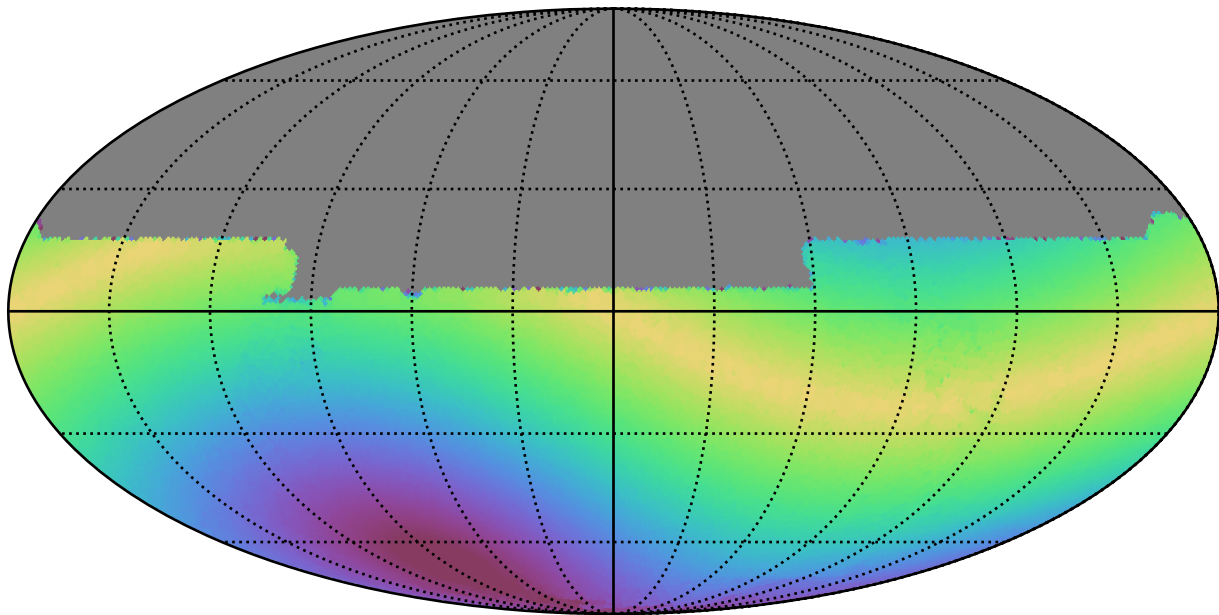
early_u_fpextra2.0_v3.4_10yrs All sky y band: Max solarElong
