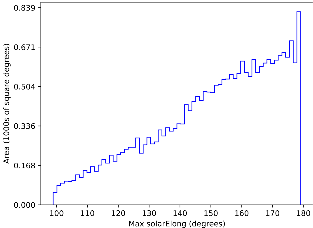
early_u_fpextra2.0_v3.4_10yrs All sky y band: Max solarElong
