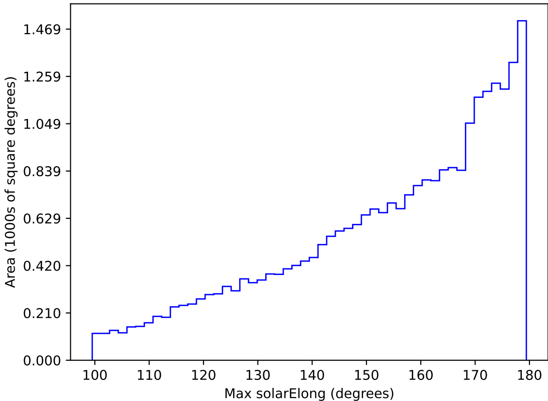
early_u_fpextra2.0_v3.4_10yrs All sky r band: Max solarElong
