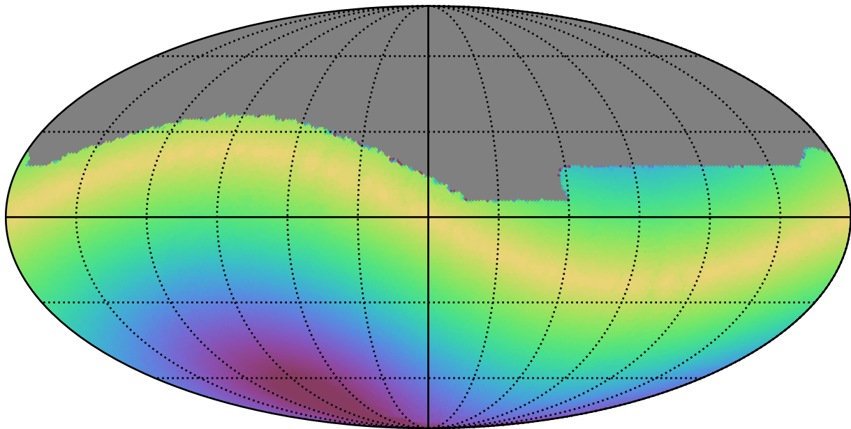
early_u_fpextra2.0_v3.4_10yrs All sky i band: Max solarElong
