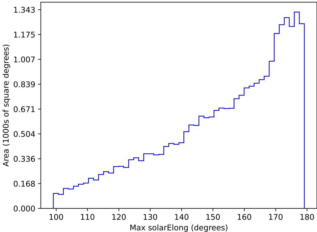
early_u_fpextra2.0_v3.4_10yrs All sky g band: Max solarElong
