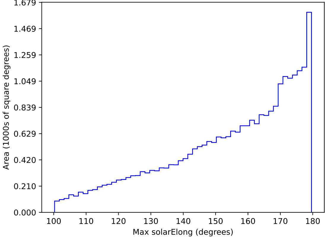
early_u_fpextra2.0_v3.4_10yrs All sky all bands: Max solarElong
