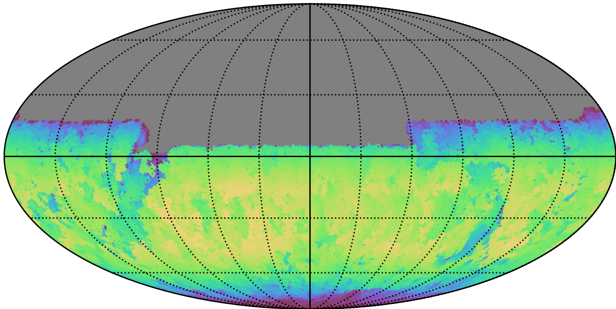
early_u_fpextra2.0_v3.4_10yrs Yr 1 y band: Max skyBrightness
