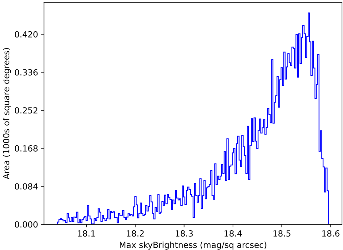
early_u_fpextra2.0_v3.4_10yrs Yr 1 y band: Max skyBrightness
