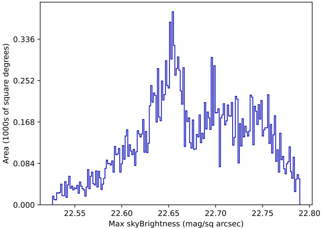
early_u_fpxextra2.0_v3.4_10yrs Yr 1 u band: Max skyBrightness
