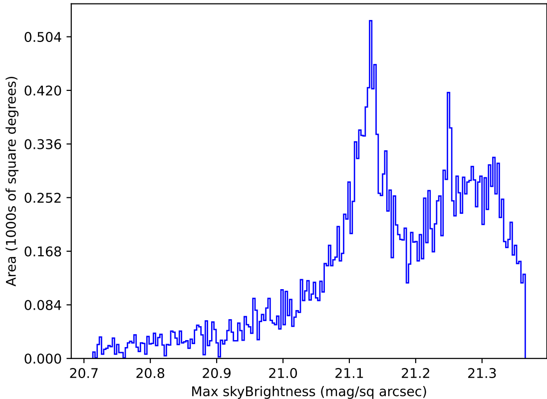
early_u_fpextra2.0_v3.4_10yrs Yr 1 r band: Max skyBrightness
