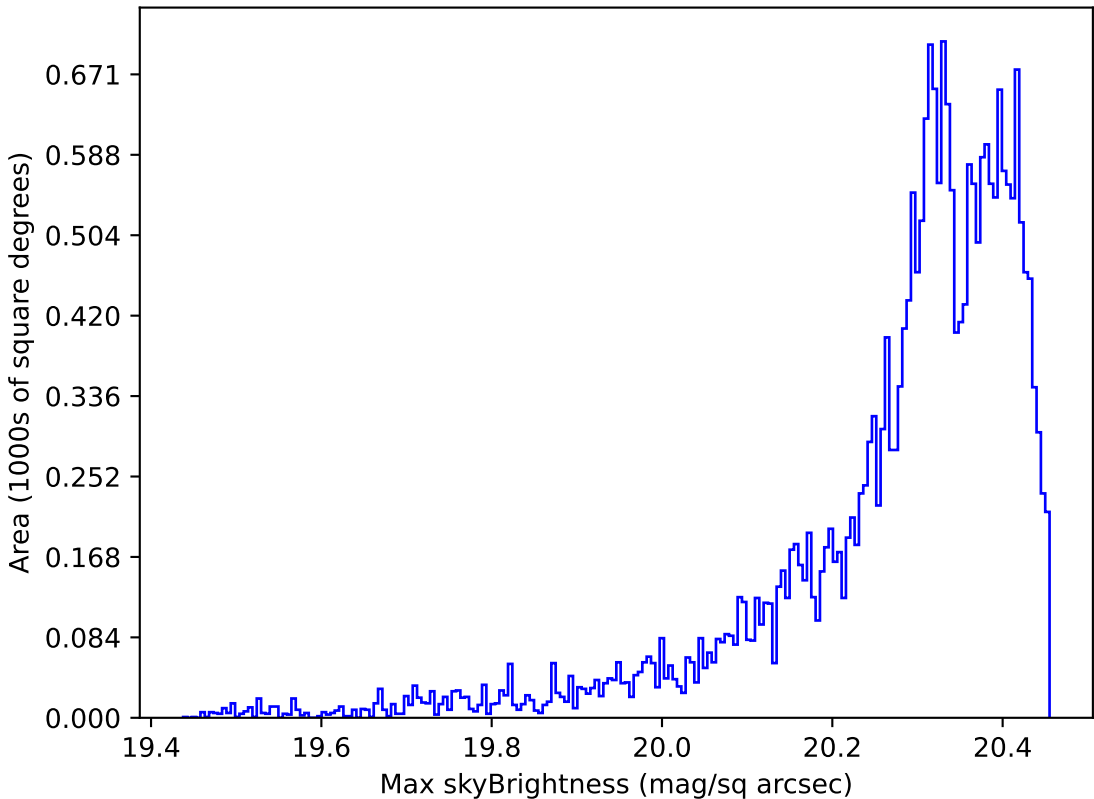
early_u_fpextra2.0_v3.4_10yrs Yr 1 i band: Max skyBrightness
