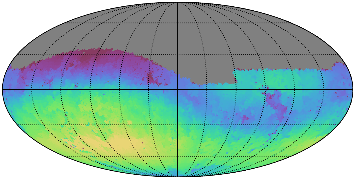
early_u_fpextra2.0_v3.4_10yrs Yr 1 g band: Max skyBrightness
