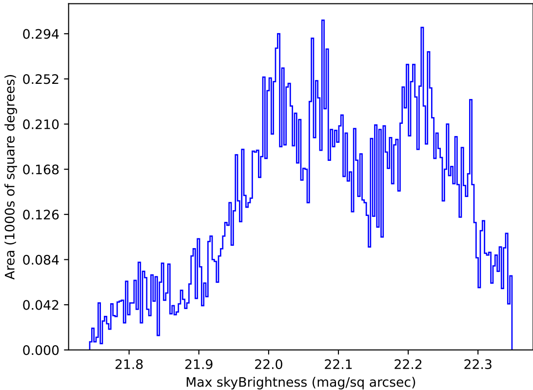
early_u_fpextra2.0_v3.4_10yrs Yr 1 g band: Max skyBrightness
