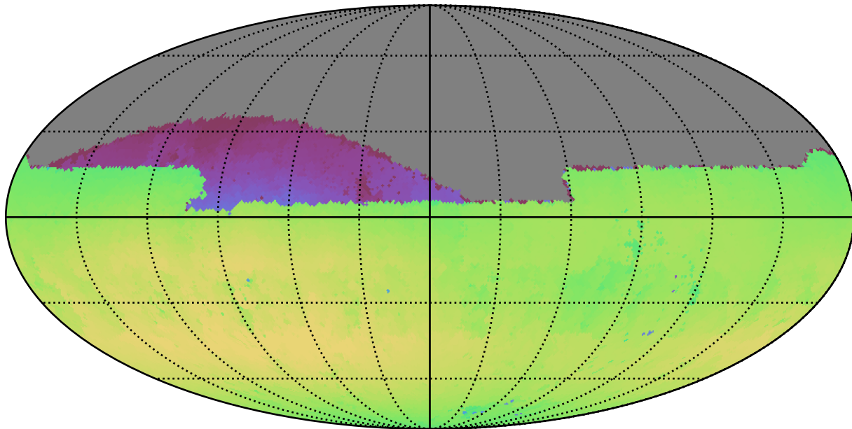
early_u_fpextra2.0_v3.4_10yrs Yr 1 all bands: Max skyBrightness
