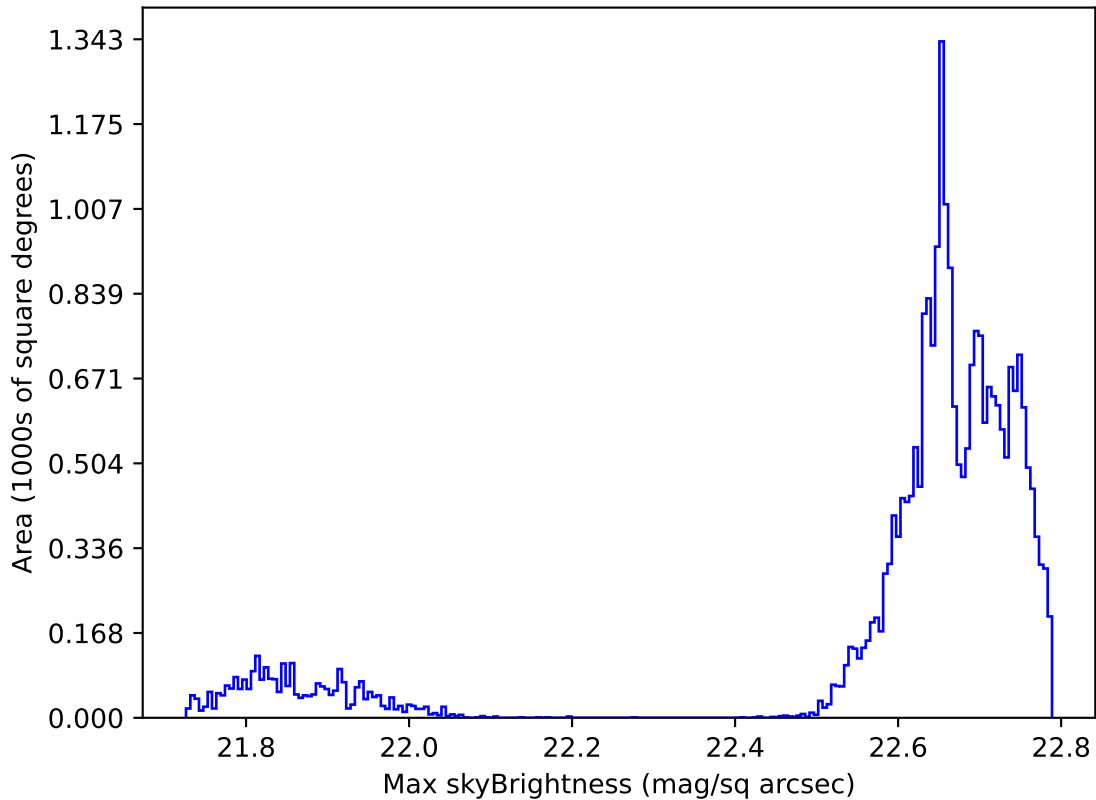
early_u_fpextra2.0_v3.4_10yrs Yr 1 all bands: Max skyBrightness
