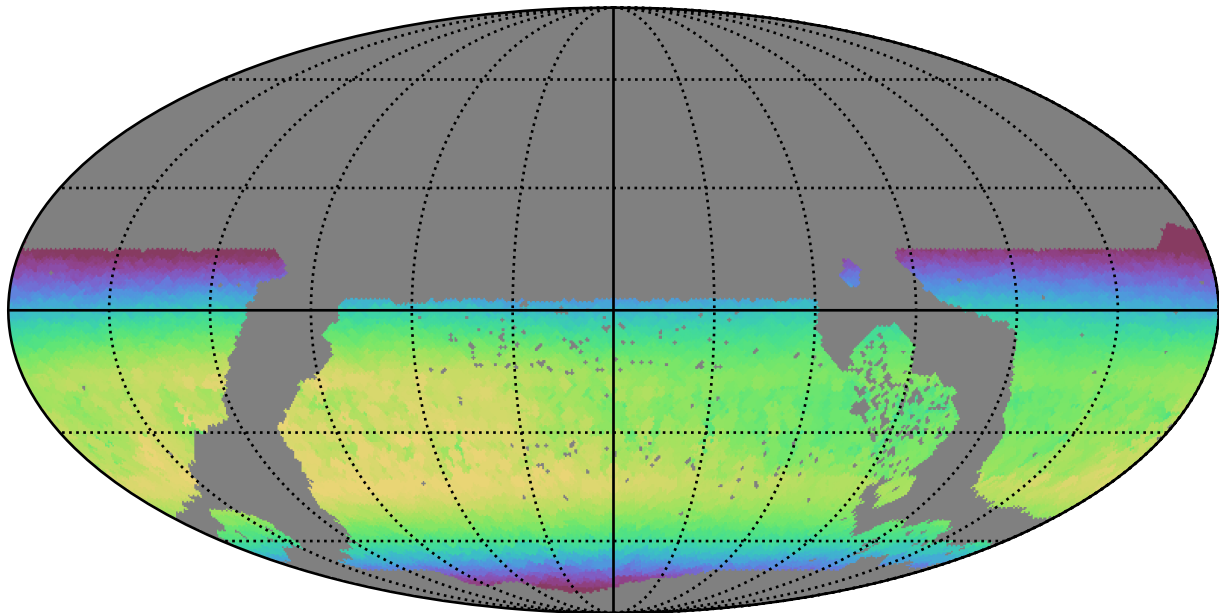
early_u_fpextra2.0_v3.4_10yrs WFD z band: Max skyBrightness
