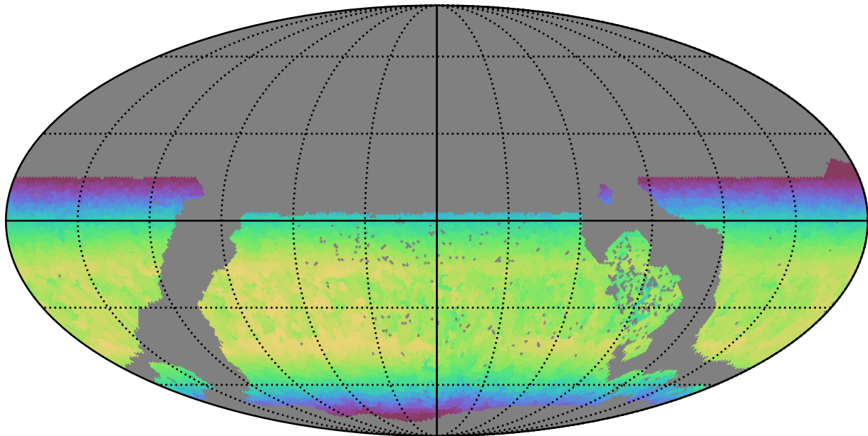
early_u_fpextra2.0_v3.4_10yrs WFD y band: Max skyBrightness
