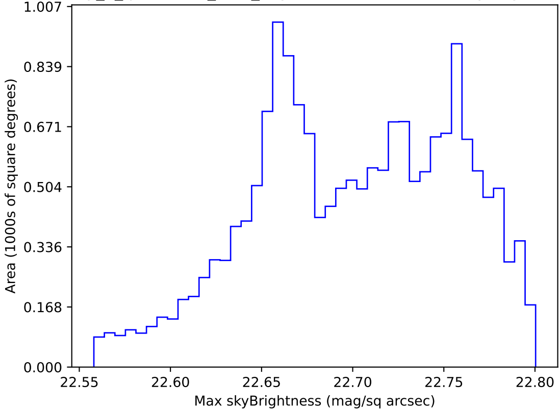
early_u_fpextra2.0_v3.4_10yrs WFD u band: Max skyBrightness
