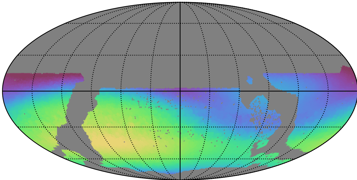
early_u_fpextra2.0_v3.4_10yrs WFD r band: Max skyBrightness
