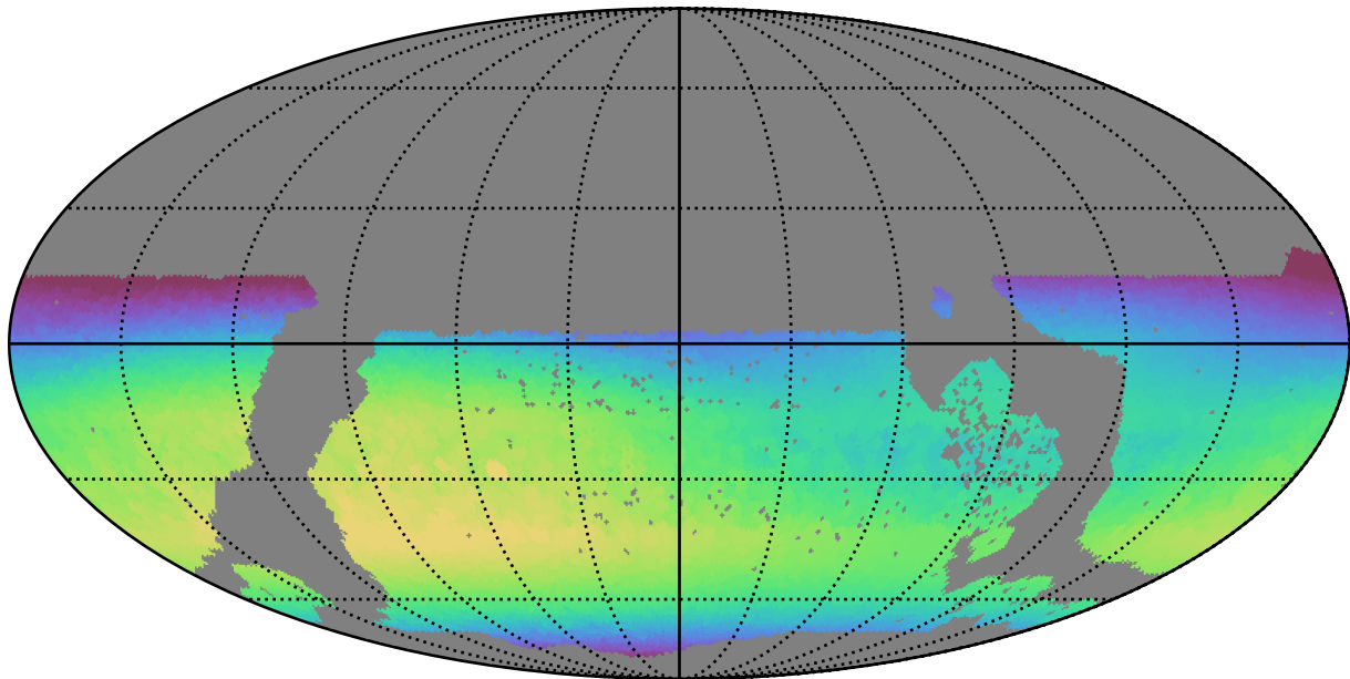
early_u_fpextra2.0_v3.4_10yrs WFD i band: Max skyBrightness
