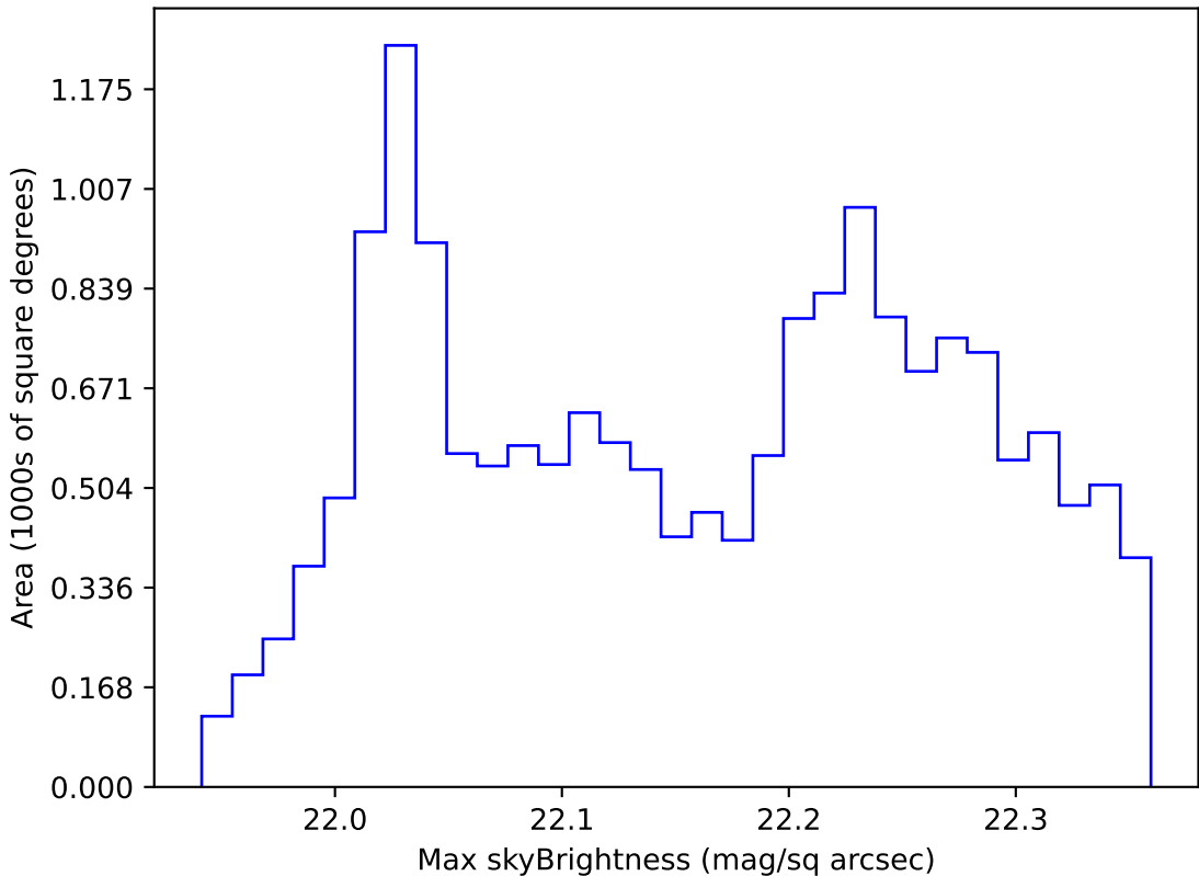
early_u_fpextra2.0_v3.4_10yrs WFD g band: Max skyBrightness
