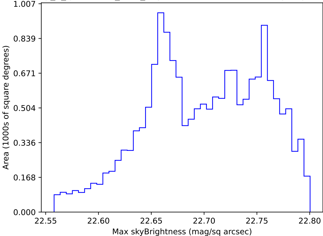
early_u_fpextra2.0_v3.4_10yrs WFD all bands: Max skyBrightness
