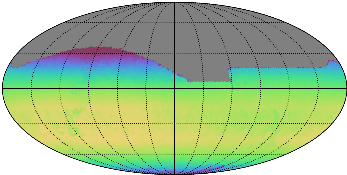
early_u_fpextra2.0_v3.4_10yrs All sky z band: Max skyBrightness
