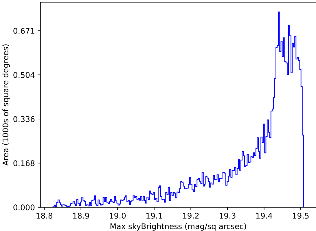
early_u_fpextra2.0_v3.4_10yrs All sky z band: Max skyBrightness
