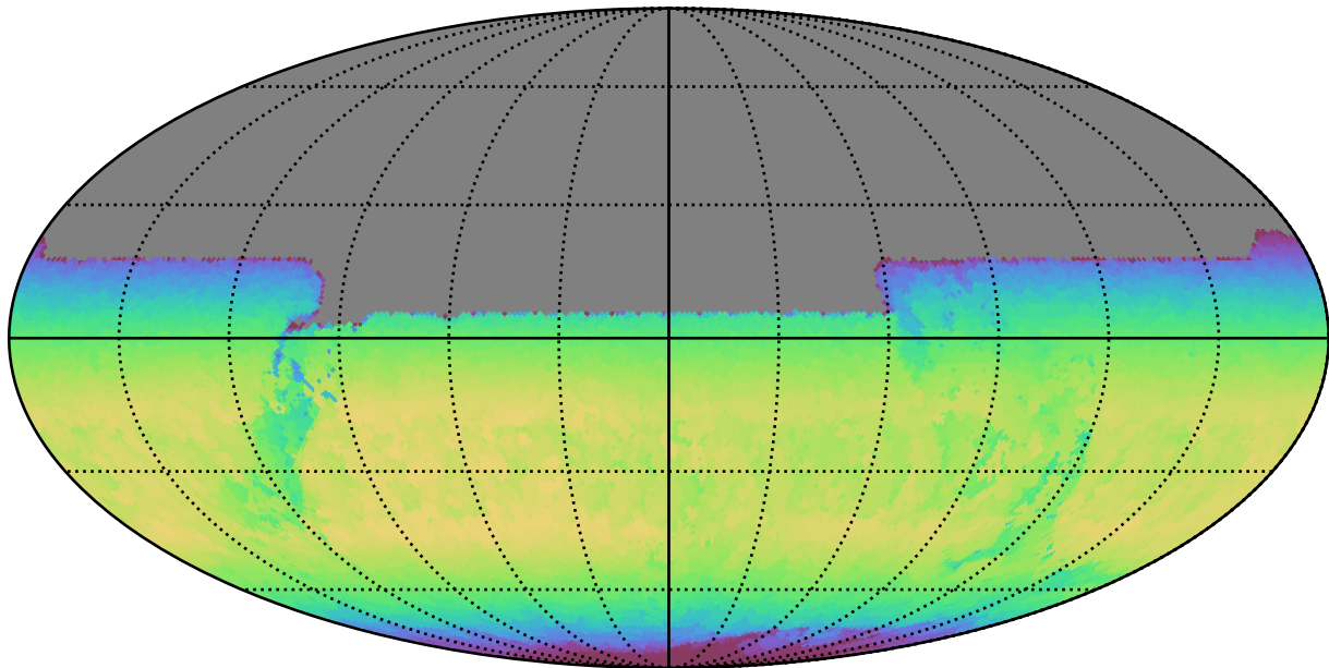
early_u_fpextra2.0_v3.4_10yrs All sky y band: Max skyBrightness
