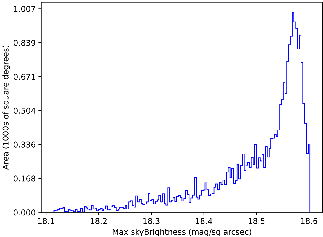
early_u_fpextra2.0_v3.4_10yrs All sky y band: Max skyBrightness
