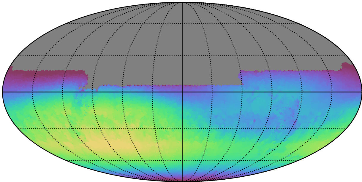
early_u_fpextra2.0_v3.4_10yrs All sky u band: Max skyBrightness
