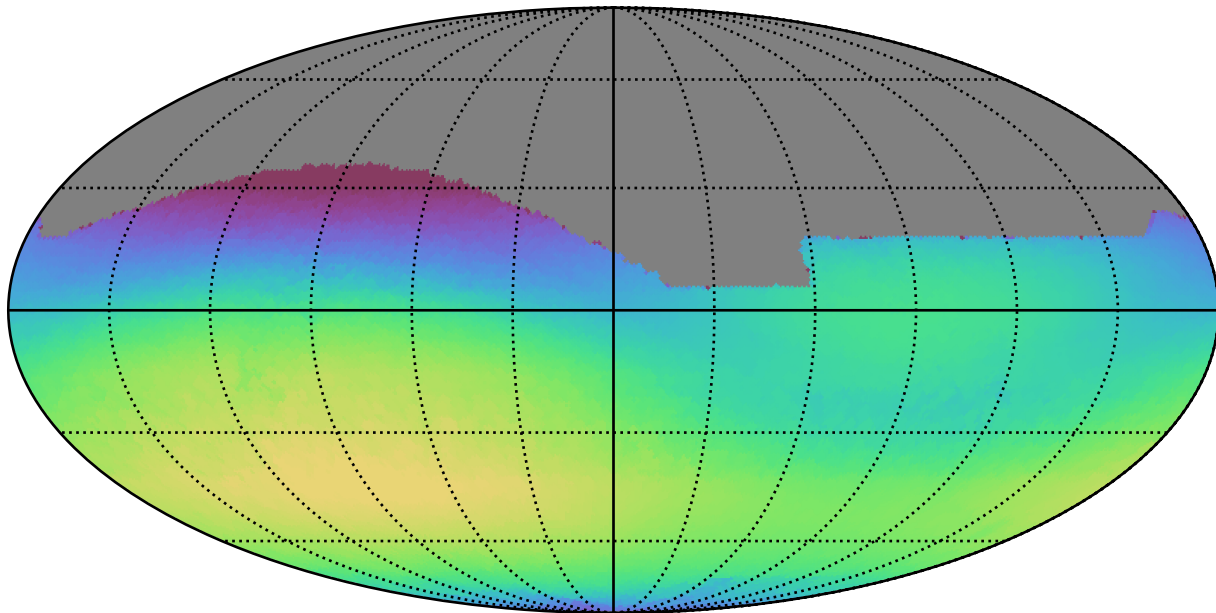
early_u_fpextra2.0_v3.4_10yrs All sky r band: Max skyBrightness
