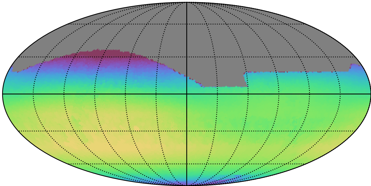
early_u_fpextra2.0_v3.4_10yrs All sky i band: Max skyBrightness
